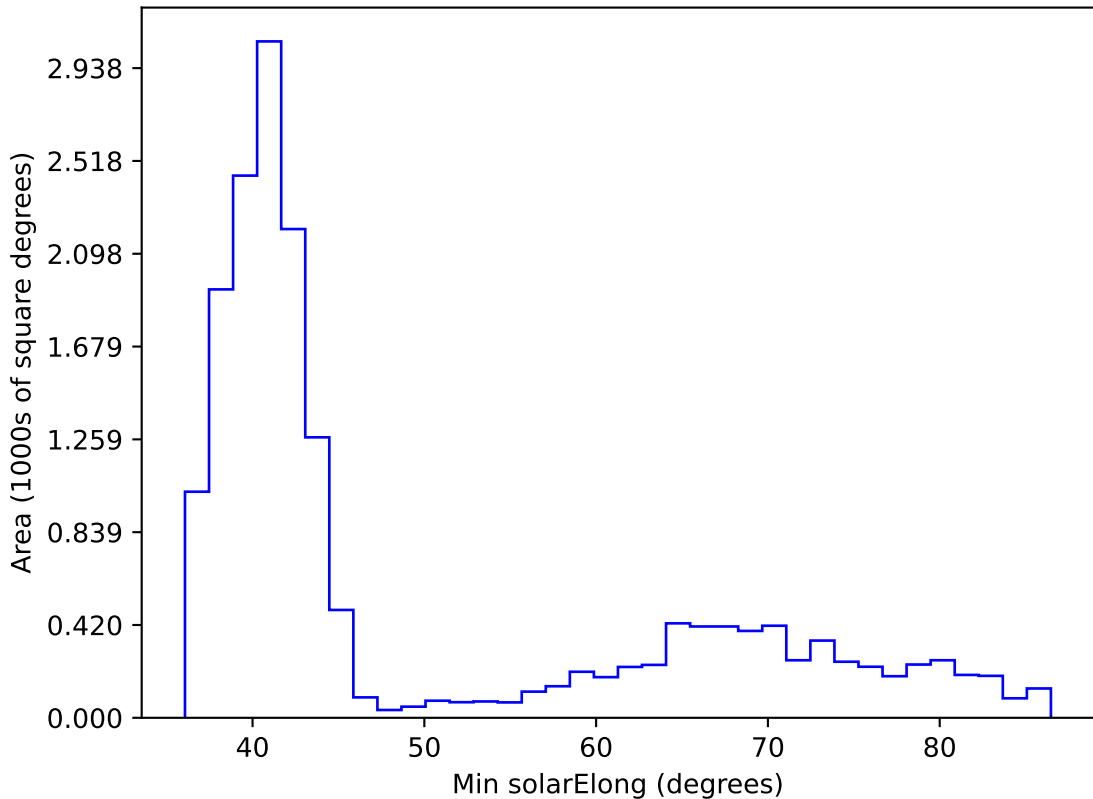
internal_u_expt60_nscale1.2v3.4_10yrs WFD i band: Min solarElong
