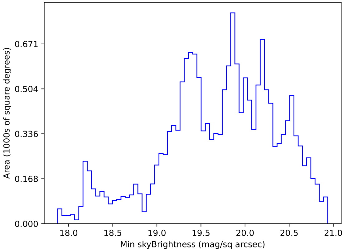
internal_u_expt60_nscale1.2v3.4_10yrs WFD g band: Min skyBrightness
