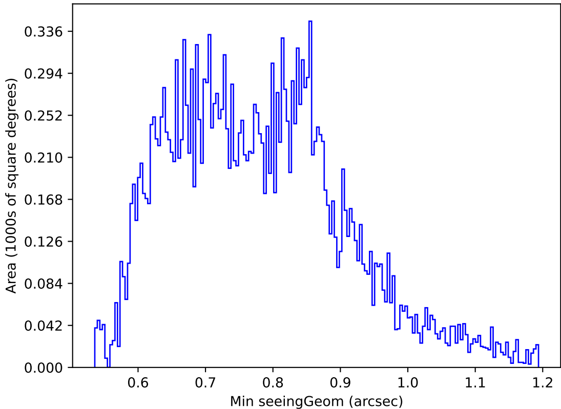
internal_u_expt60_nscale1.2v3.4_10yrs Yr 1 u band: Min seeingGeom
