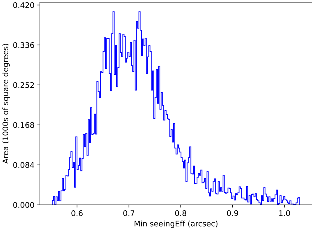
internal_u_expt60_nscale1.2v3.4_10yrs Yr 1 y band: Min seeingEff
