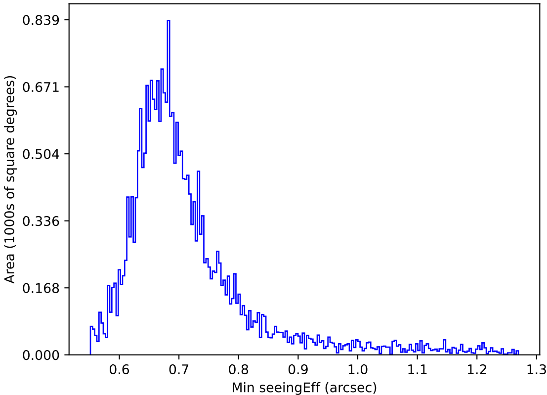
internal_u_expt60_nscale1.2v3.4_10yrs Yr 1 i band: Min seeingEff
