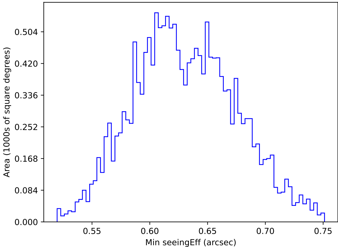
internal_u_expt60_nscale1.2v3.4_10yrs WFD y band: Min seeingEff
