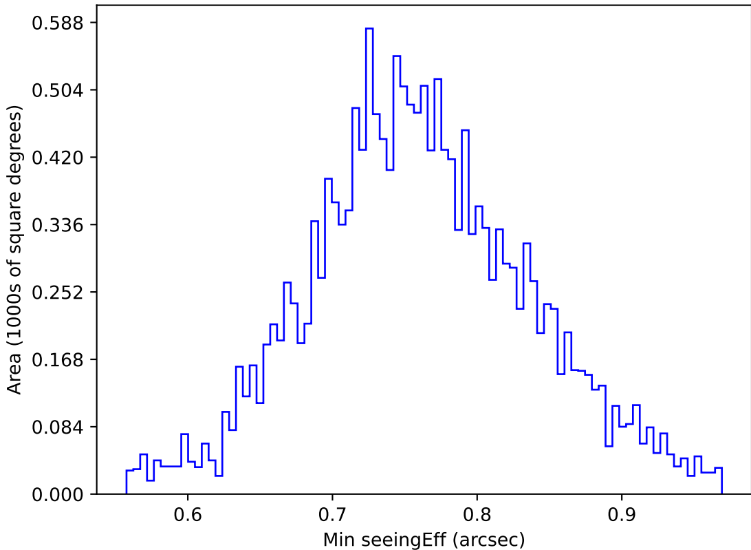
internal_u_expt60_nscale1.2v3.4_10yrs WFD u band: Min seeingEff
