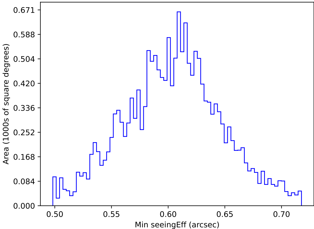
internal_u_expt60_nscale1.2v3.4_10yrs WFD i band: Min seeingEff
