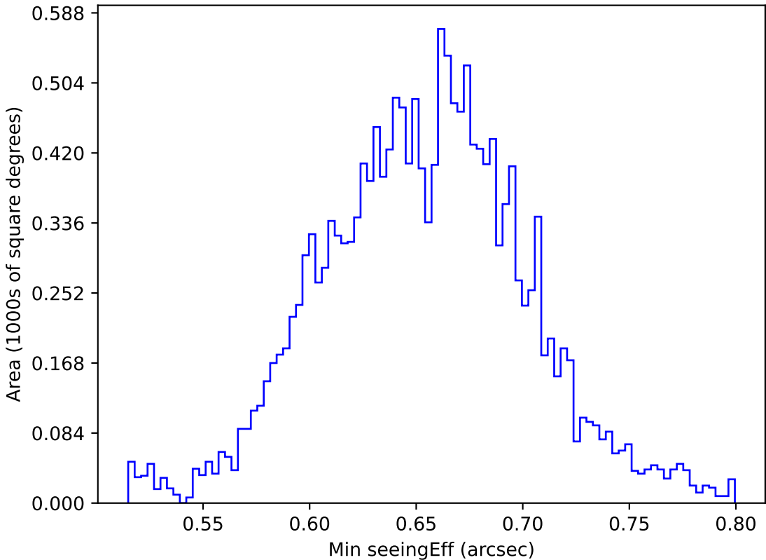
internal_u_expt60_nscale1.2v3.4_10yrs WFD g band: Min seeingEff
