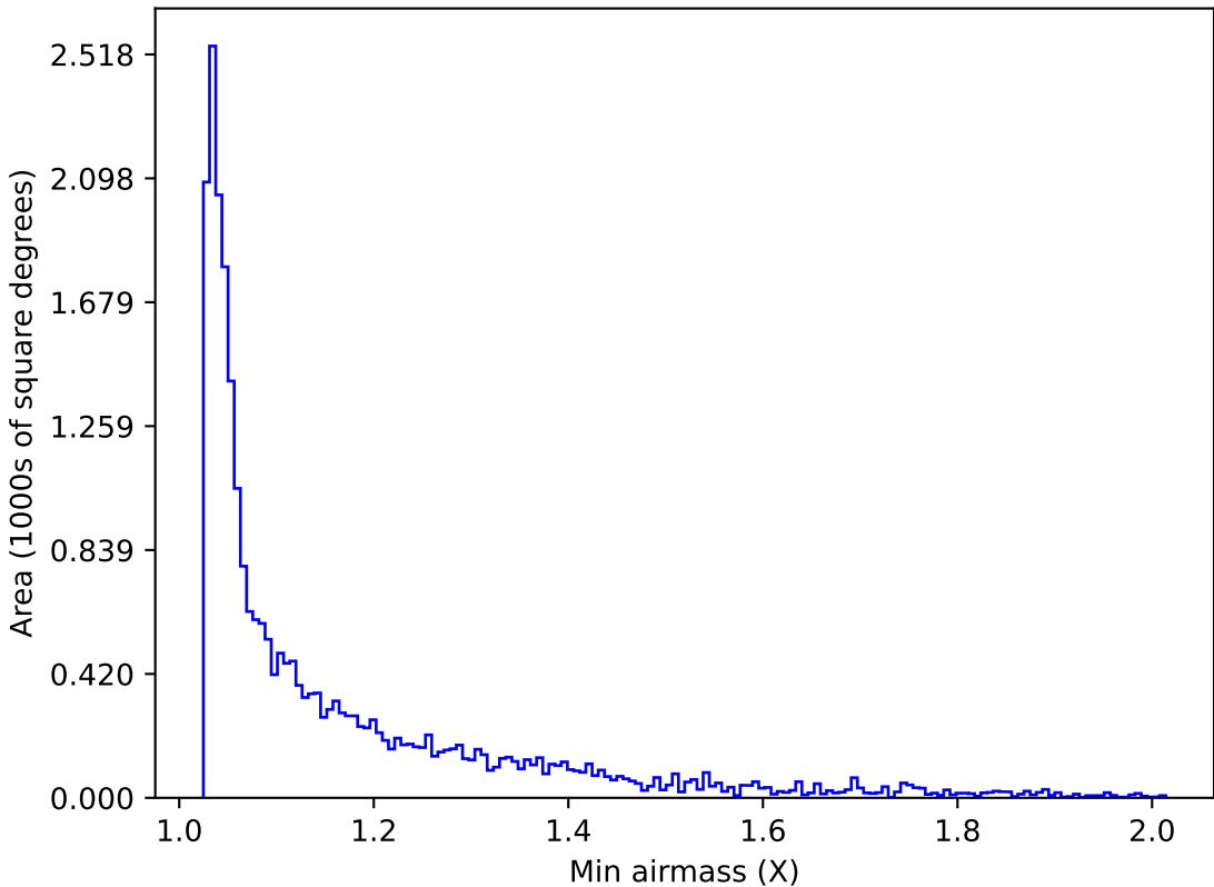
internal_u_expt60_nscale1.2v3.4_10yrs Yr 1 z band: Min airmass
