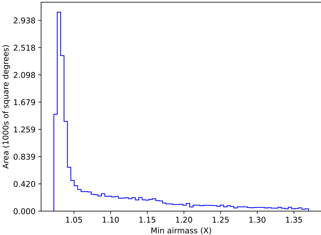
internal_u_expt60_nscale1.2v3.4_10yrs WFD y band: Min airmass
