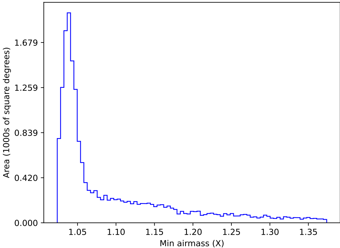
internal_u_expt60_nscale1.2v3.4_10yrs WFD u band: Min airmass
