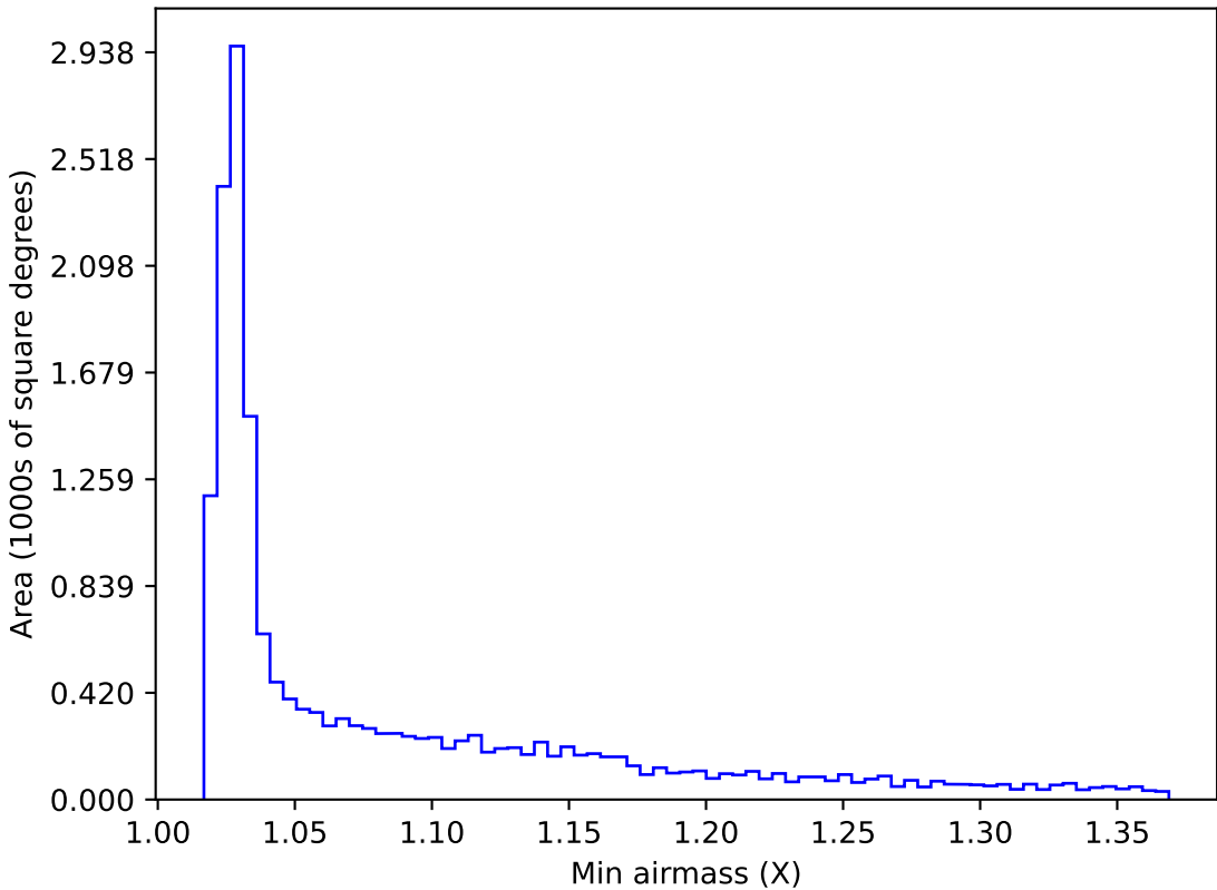
internal_u_expt60_nscale1.2v3.4_10yrs WFD r band: Min airmass
