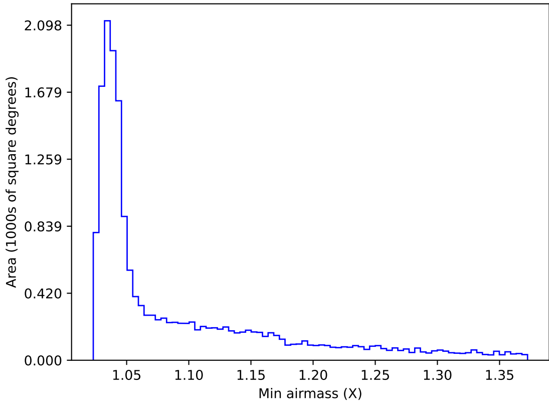
internal_u_expt60_nscale1.2v3.4_10yrs WFD g band: Min airmass
