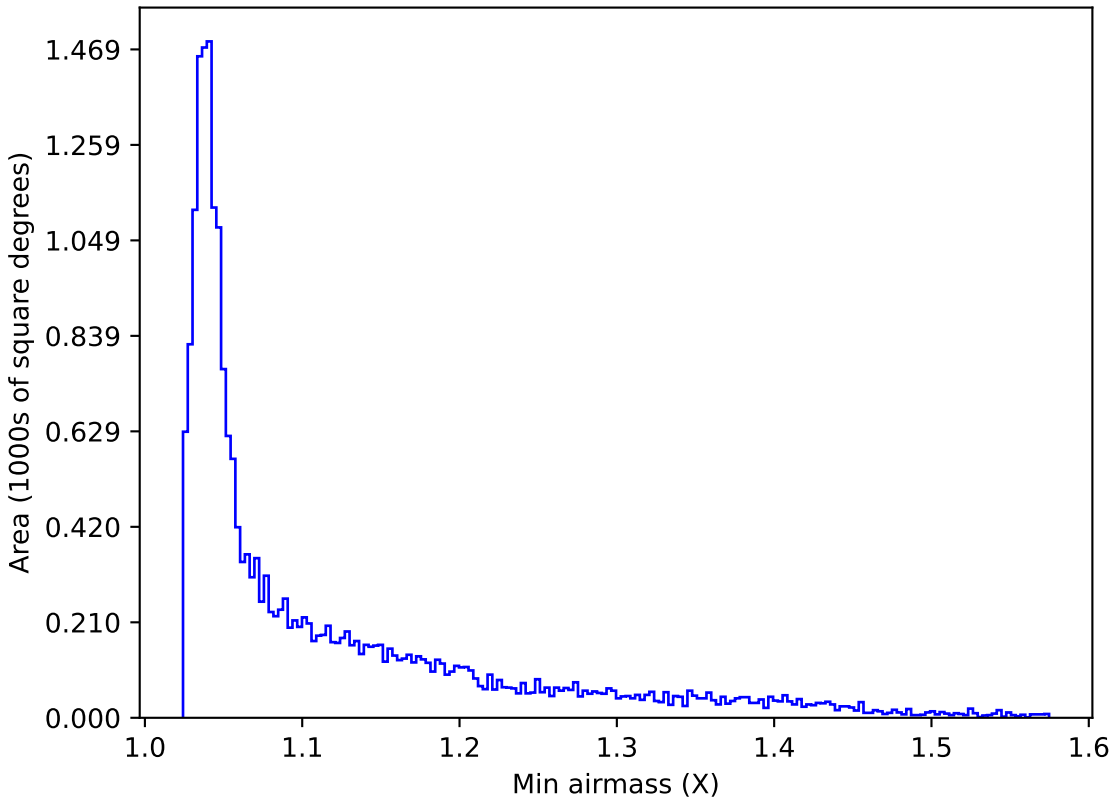
internal_u_expt60_nscale1.2v3.4_10yrs All sky u band: Min airmass
