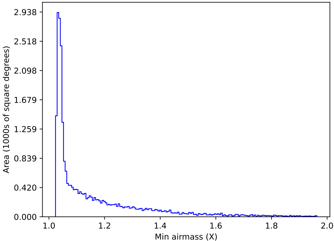
internal_u_expt60_nscale1.2v3.4_10yrs All sky g band: Min airmass
