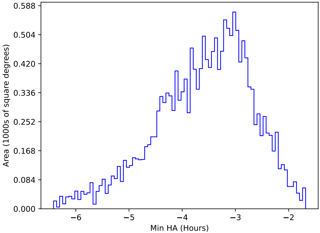
internal_u_expt60_nscale1.2v3.4_10yrs WFD y band: Min HA
