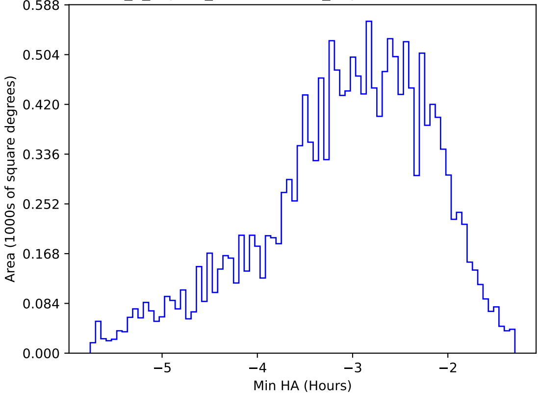
internal_u_expt60_nscale1.2v3.4_10yrs WFD u band: Min HA
