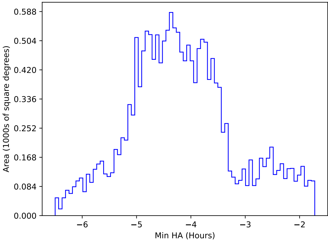
internal_u_expt60_nscale1.2v3.4_10yrs WFD g band: Min HA
