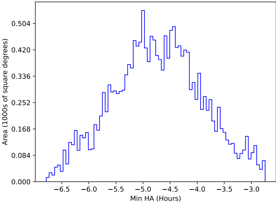
internal_u_expt60_nscale1.2v3.4_10yrs WFD all bands: Min HA
