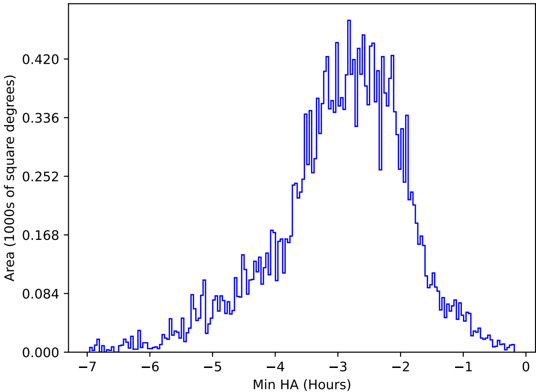
internal_u_expt60_nscale1.2v3.4_10yrs All sky u band: Min HA
