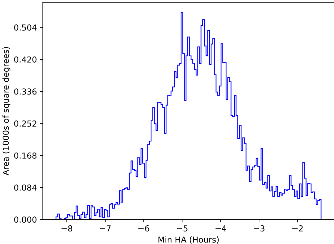
internal_u_expt60_nscale1.2v3.4_10yrs All sky all bands: Min HA
