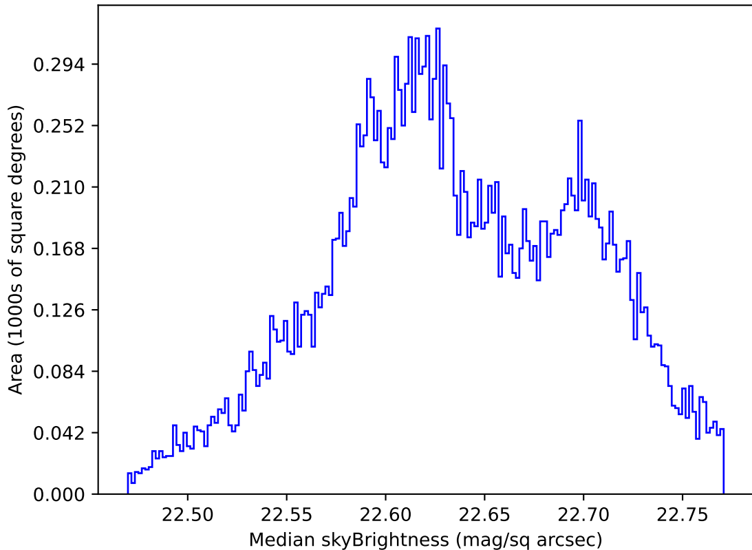
internal_u_expt60_nscale1.2v3.4_10yrs Yr 1 u band: Median skyBrightness
