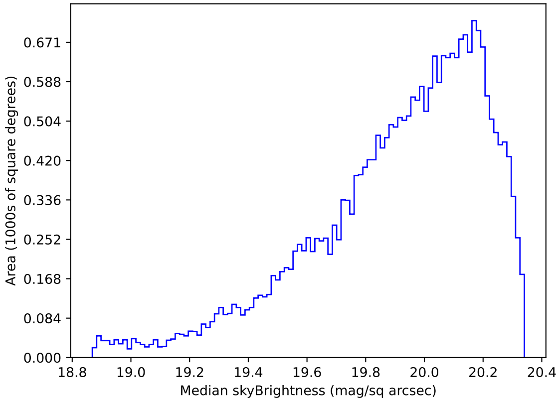
internal_u_expt60_nscale1.2v3.4_10yrs Yr 1 i band: Median skyBrightness
