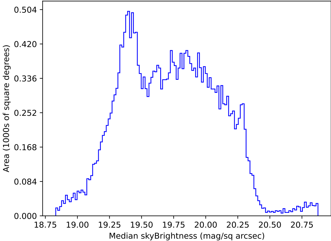
internal_u_expt60_nscale1.2v3.4_10yrs Yr 1 all bands: Median skyBrightness
