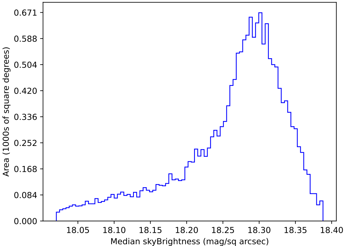
internal_u_expt60_nscale1.2v3.4_10yrs WFD y band: Median skyBrightness
