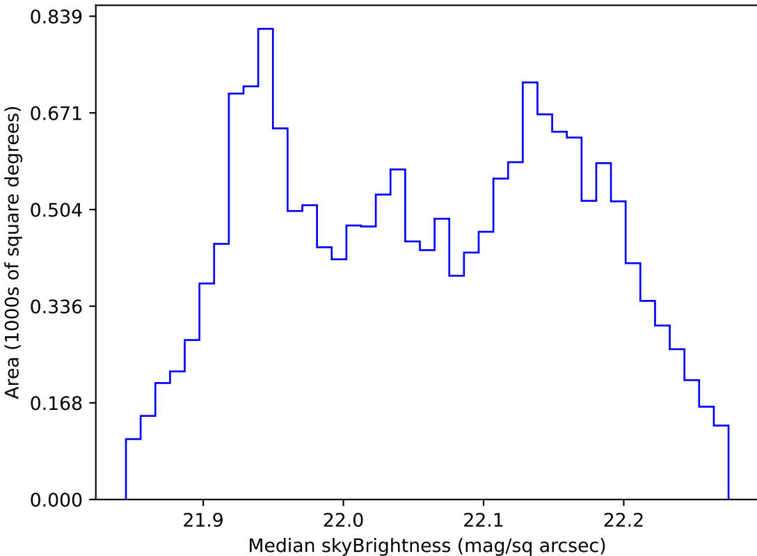
internal_u_expt60_nscale1.2v3.4_10yrs WFD g band: Median skyBrightness
