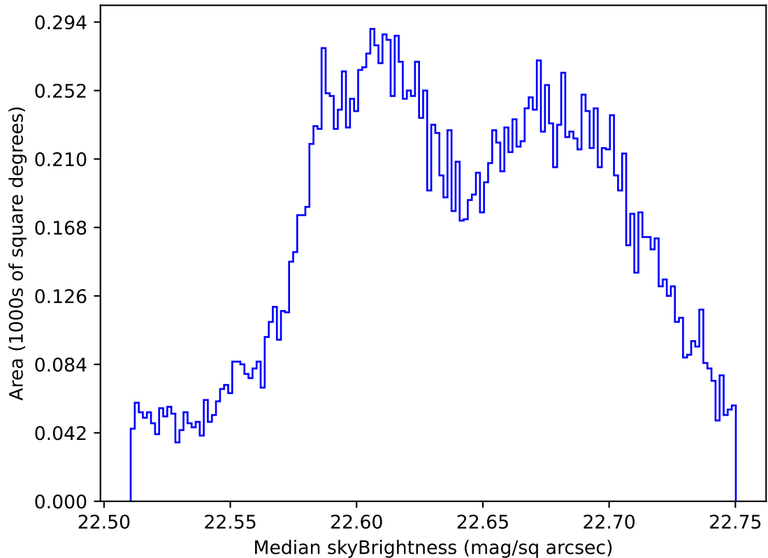
internal_u_expt60_nscale1.2v3.4_10yrs All sky u band: Median skyBrightness
