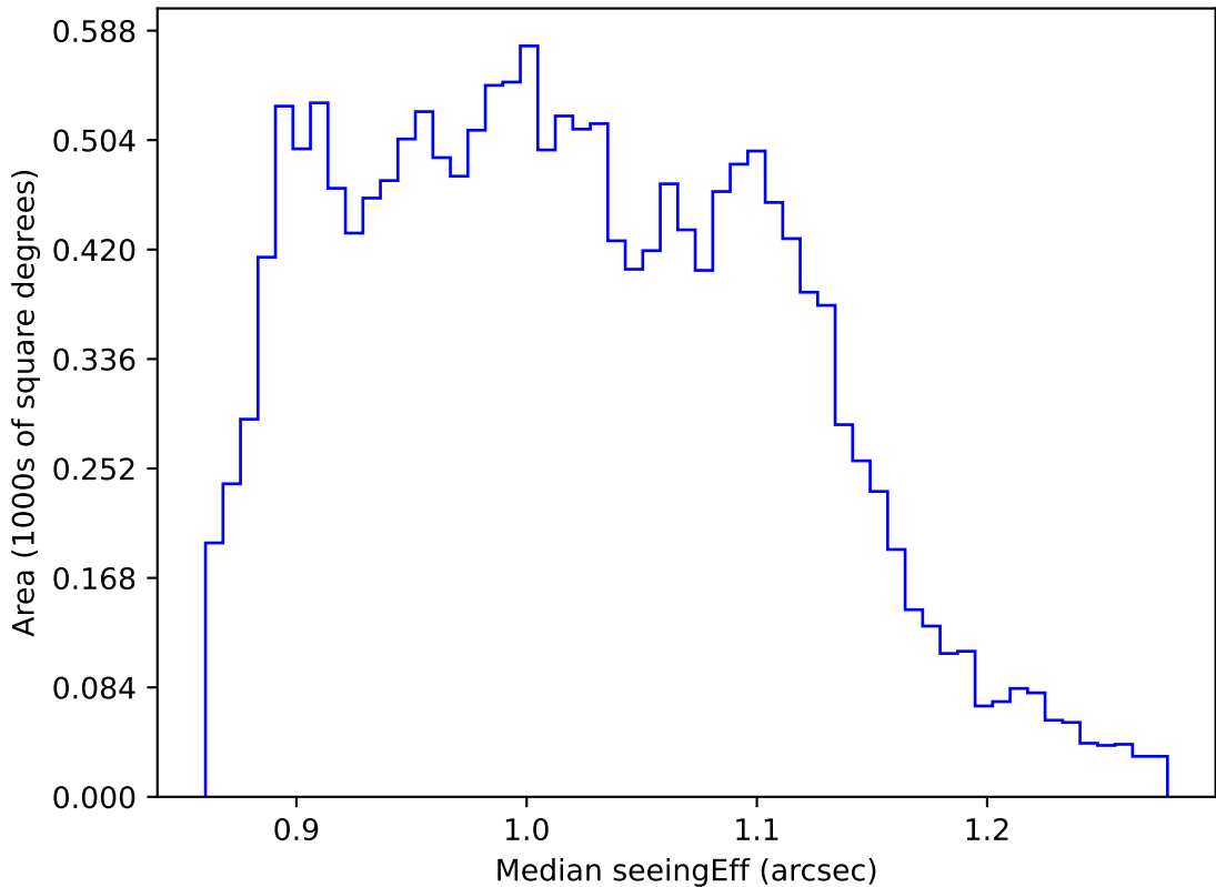
internal_u_expt60_nscale1.2v3.4_10yrs WFD r band: Median seeingEff
