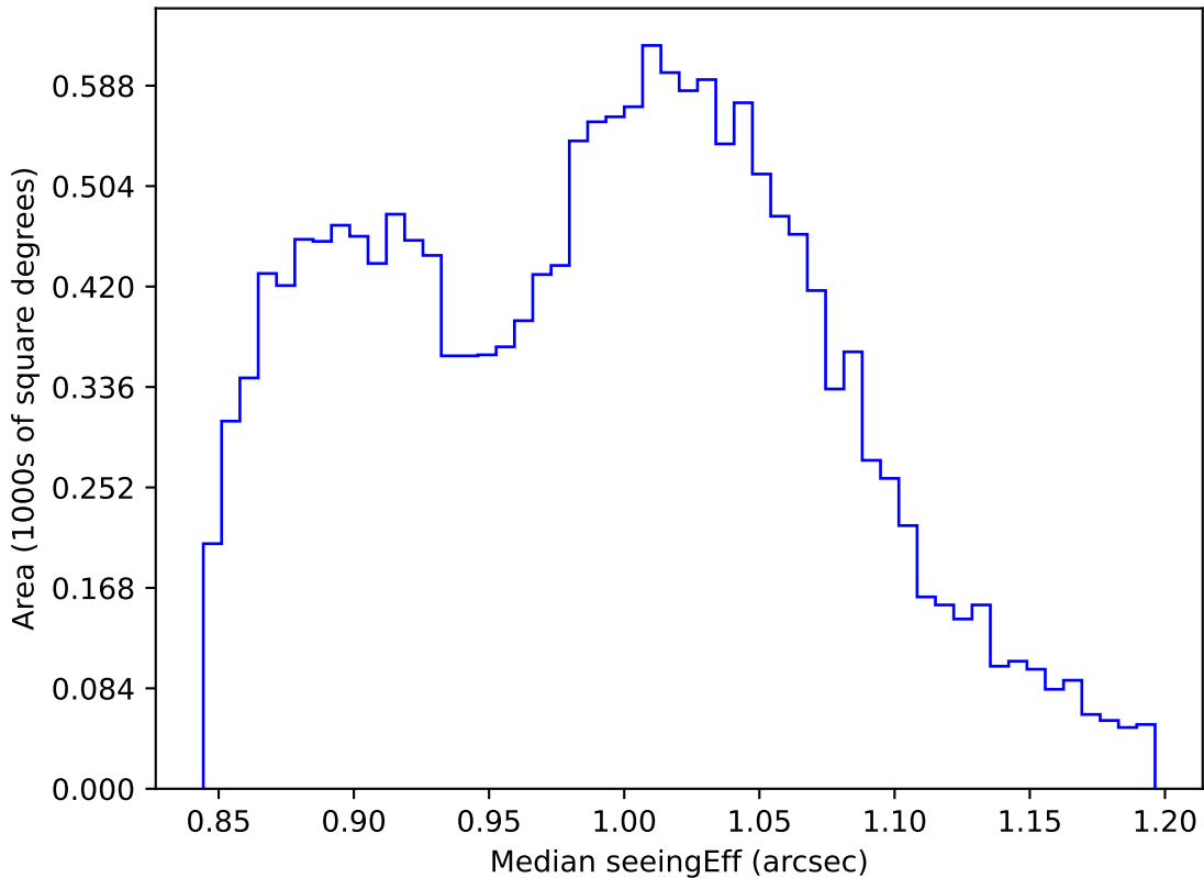
internal_u_expt60_nscale1.2v3.4_10yrs WFD i band: Median seeingEff
