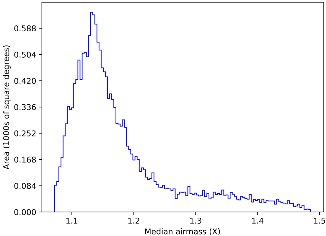
internal_u_expt60_nscale1.2v3.4_10yrs WFD g band: Median airmass
