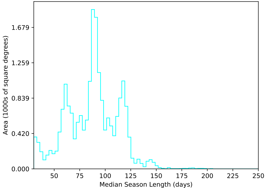
internal_u_expt60_nscale1.2v3.4_10yrs All sky u band: Median Season Length
