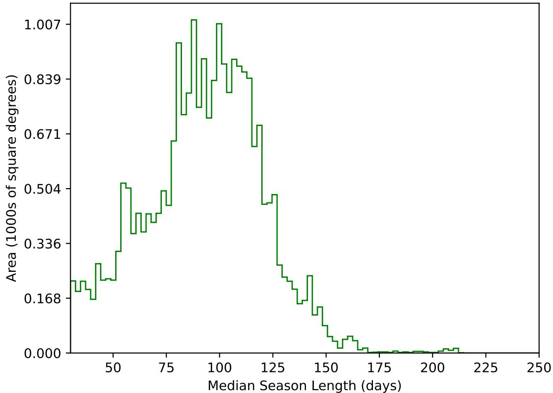
internal_u_expt60_nscale1.2v3.4_10yrs All sky g band: Median Season Length
