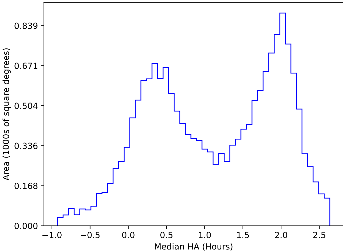
internal_u_expt60_nscale1.2v3.4_10yrs WFD u band: Median HA
