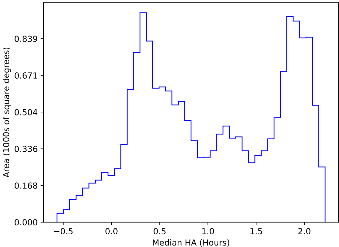
internal_u_expt60_nscale1.2v3.4_10yrs WFD all bands: Median HA
