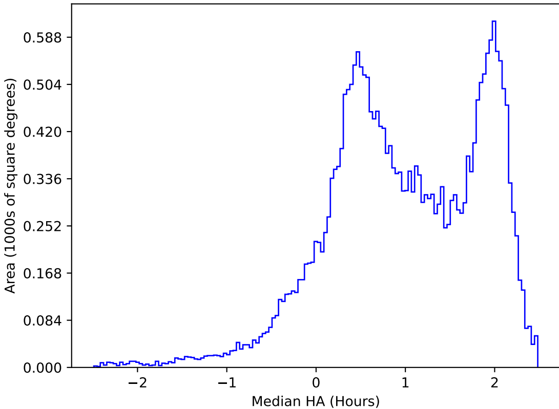
internal_u_expt60_nscale1.2v3.4_10yrs All sky z band: Median HA
