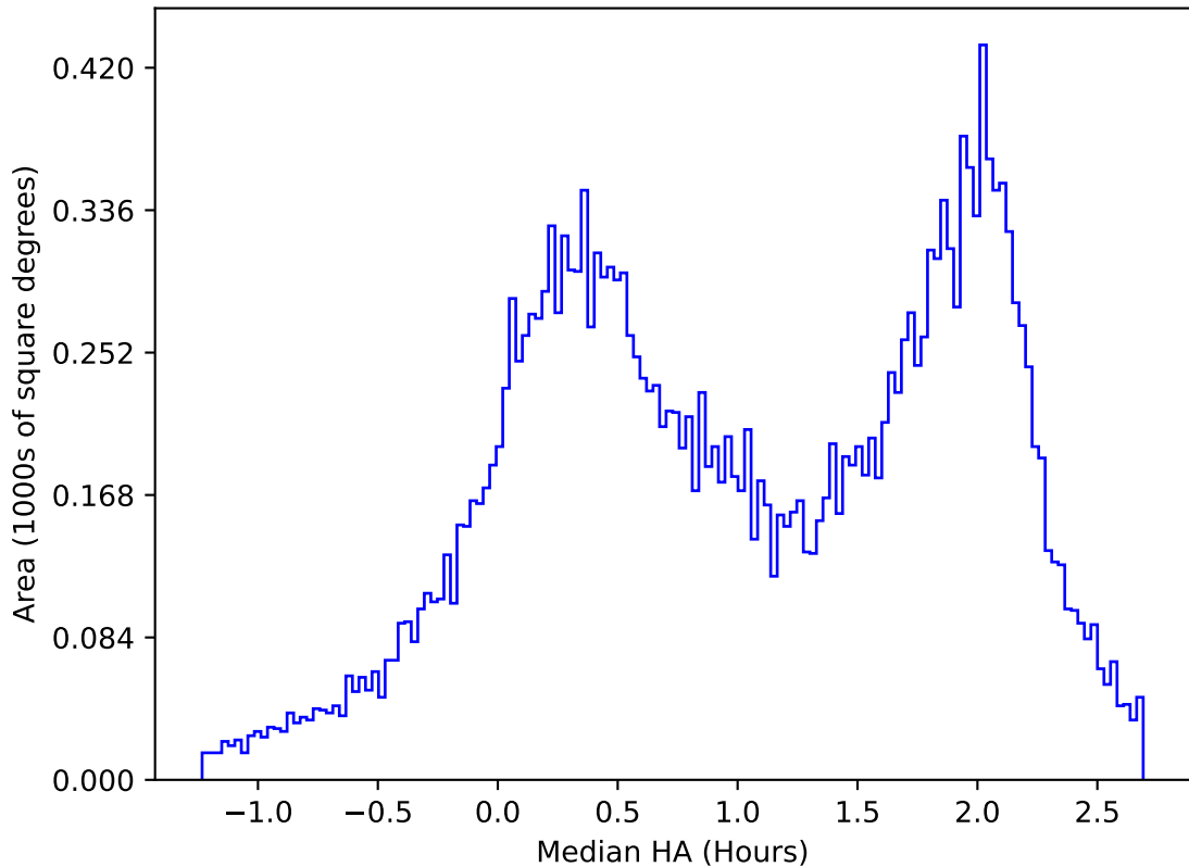
internal_u_expt60_nscale1.2v3.4_10yrs All sky u band: Median HA
