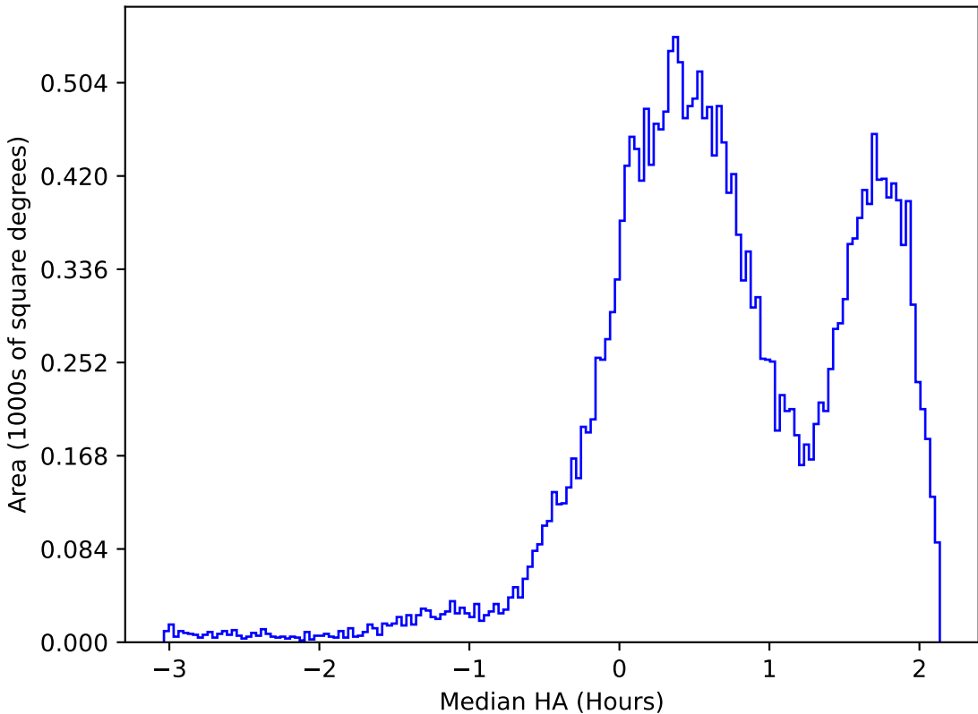
internal_u_expt60_nscale1.2v3.4_10yrs All sky r band: Median HA
