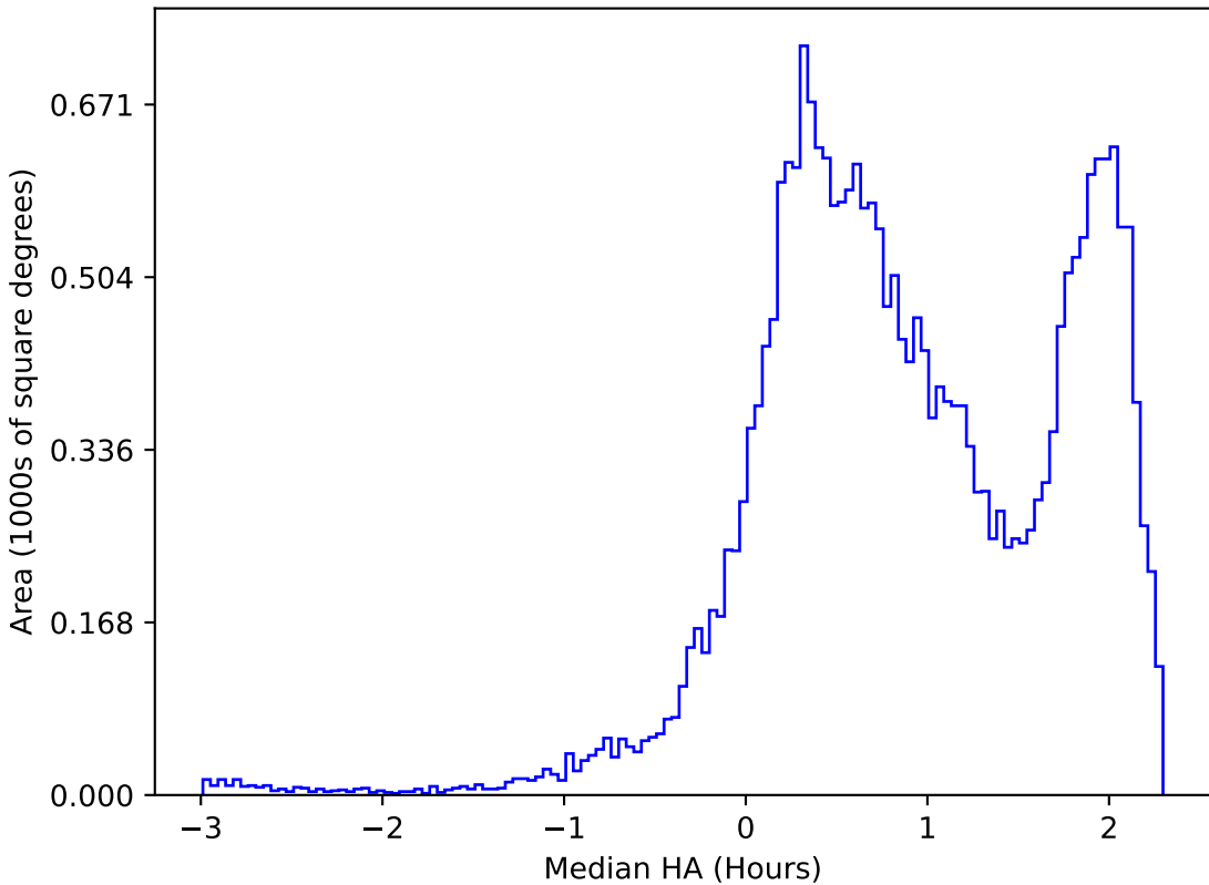
internal_u_expt60_nscale1.2v3.4_10yrs All sky i band: Median HA
