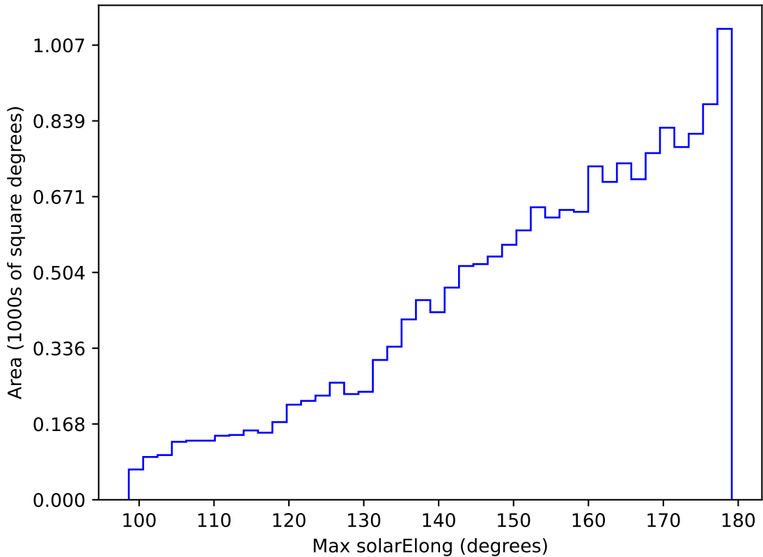
internal_u_expt60_nscale1.2v3.4_10yrs WFD y band: Max solarElong
