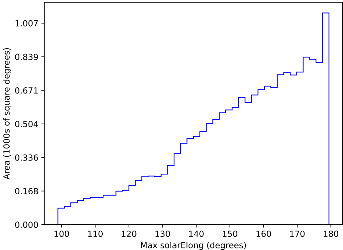
internal_u_expt60_nscale1.2v3.4_10yrs WFD r band: Max solarElong
