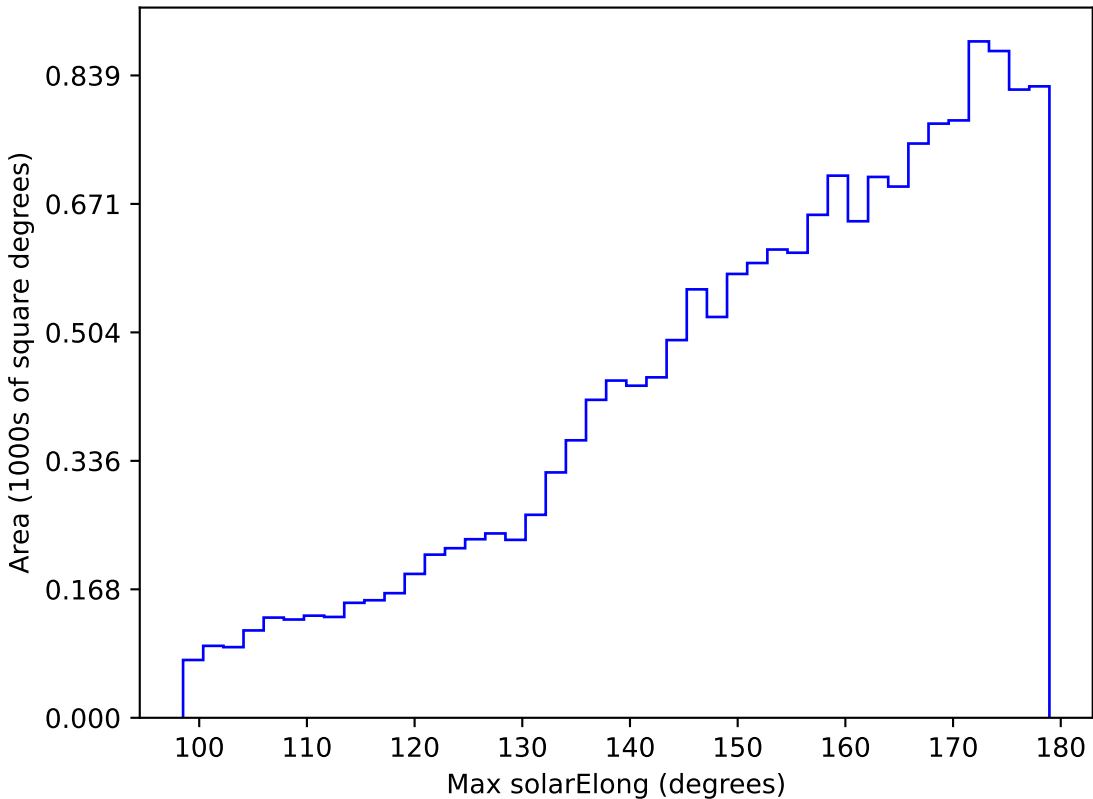
internal_u_expt60_nscale1.2v3.4_10yrs WFD g band: Max solarElong
