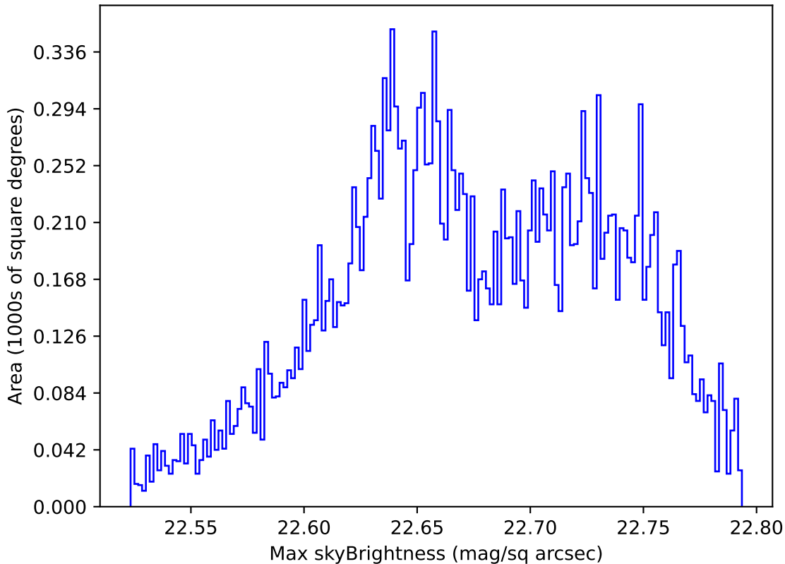
internal_u_expt60_nscale1.2v3.4_10yrs Yr 1 u band: Max skyBrightness
