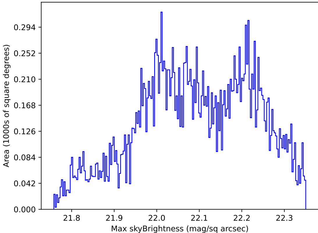
internal_u_expt60_nscale1.2v3.4_10yrs Yr 1 g band: Max skyBrightness
