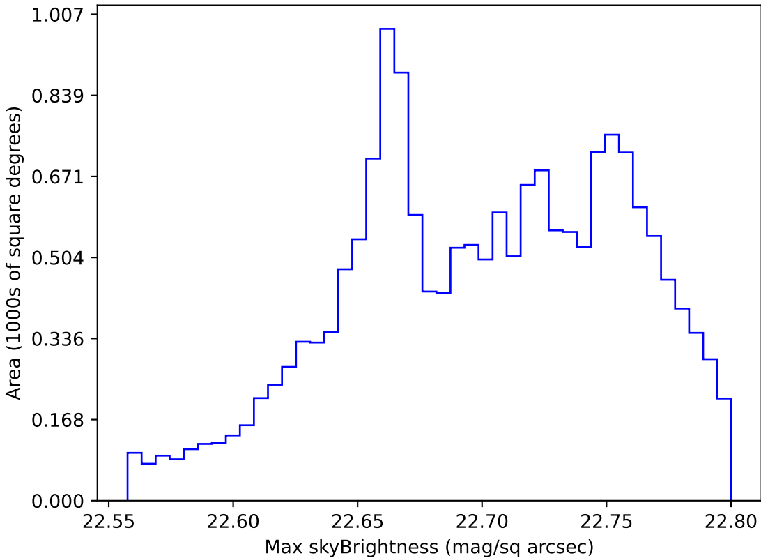
internal_u_expt60_nscale1.2v3.4_10yrs WFD all bands: Max skyBrightness
