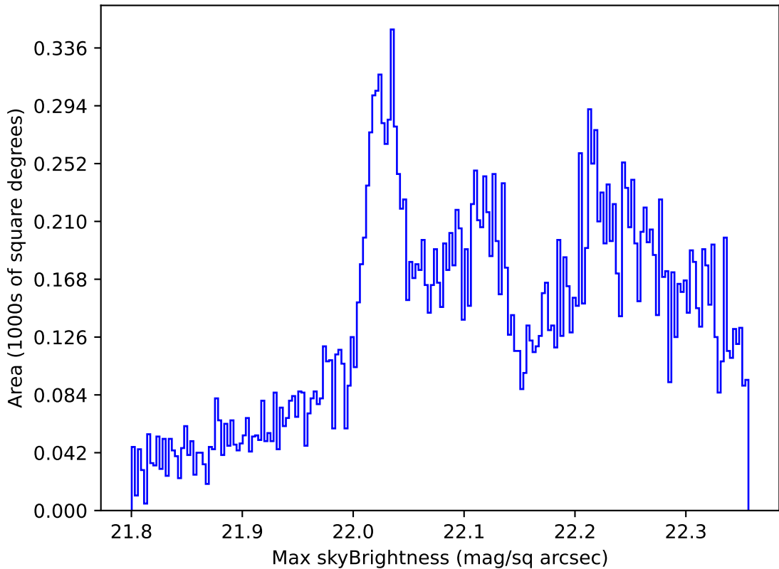
internal_u_expt60_nscale1.2v3.4_10yrs All sky g band: Max skyBrightness
