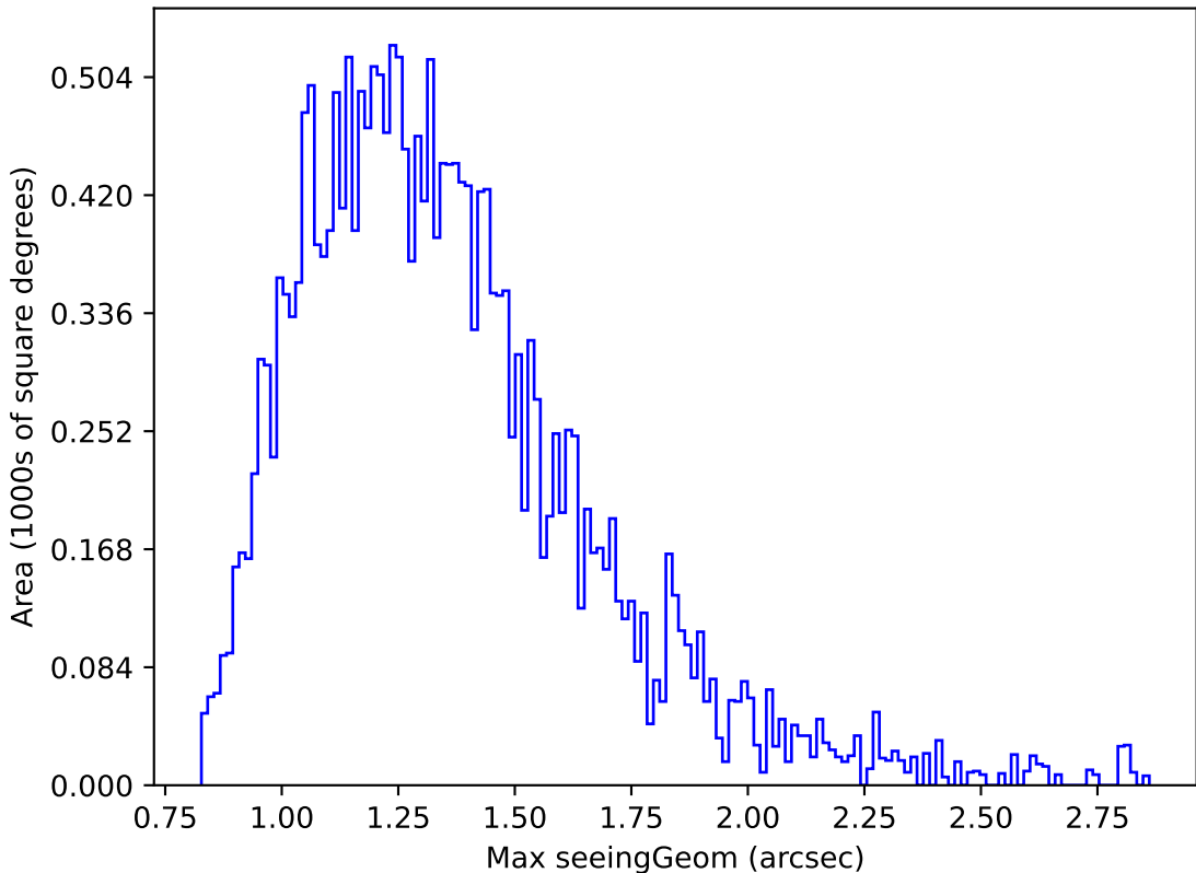
internal_u_expt60_nscale1.2v3.4_10yrs Yr 1 u band: Max seeingGeom
