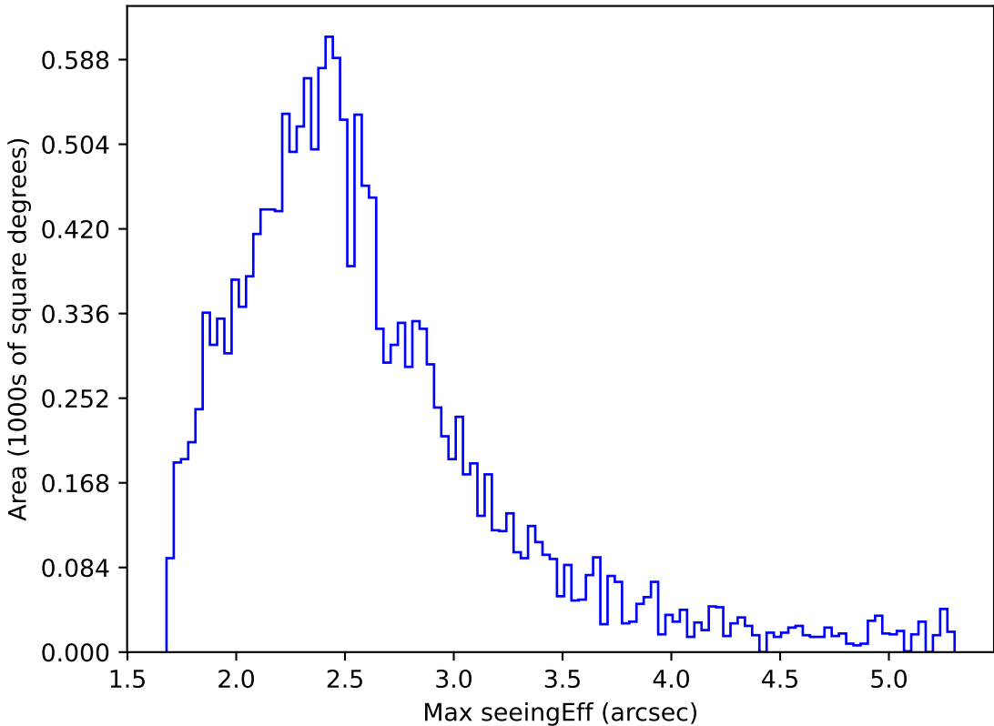
internal_u_expt60_nscale1.2v3.4_10yrs WFD z band: Max seeingEff
