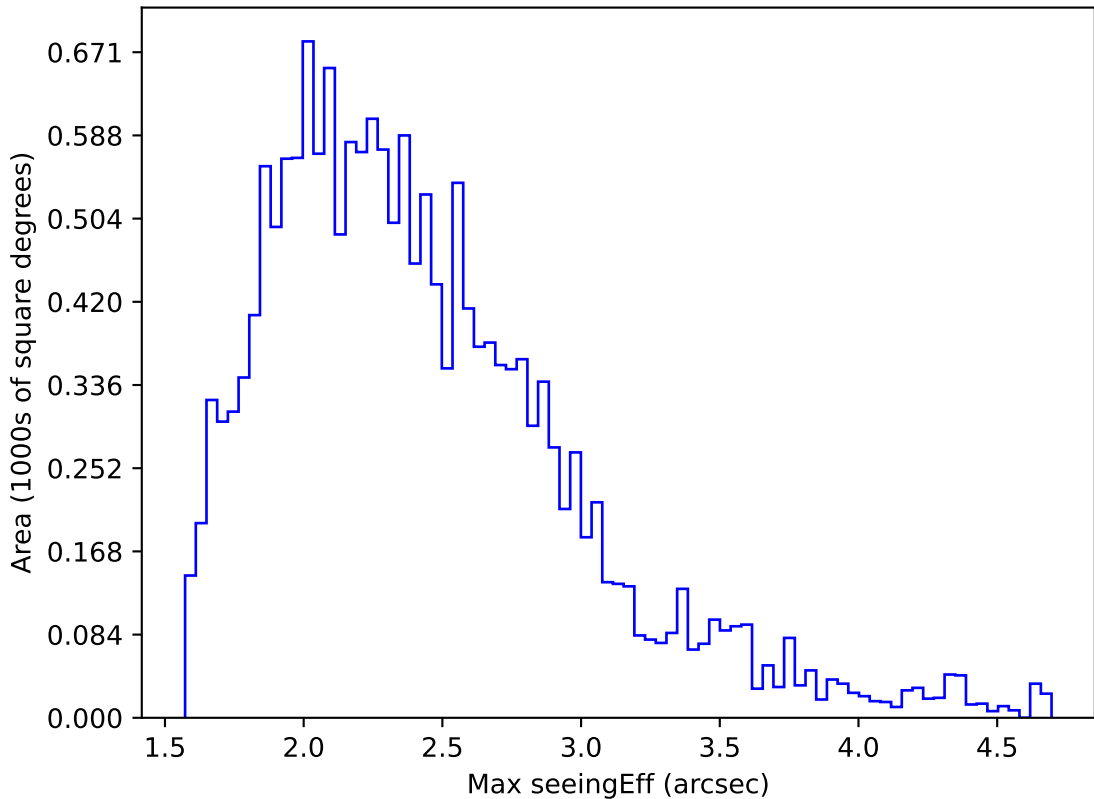
internal_u_expt60_nscale1.2v3.4_10yrs WFD y band: Max seeingEff
