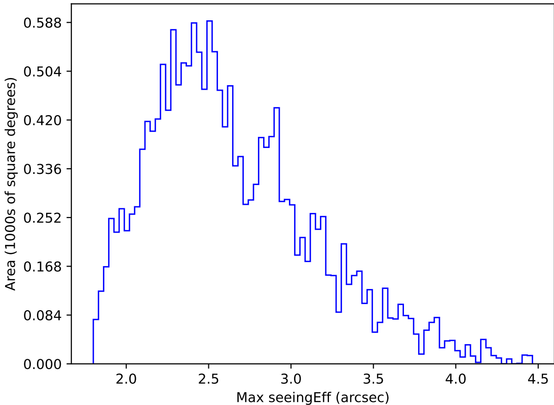
internal_u_expt60_nscale1.2v3.4_10yrs WFD r band: Max seeingEff
